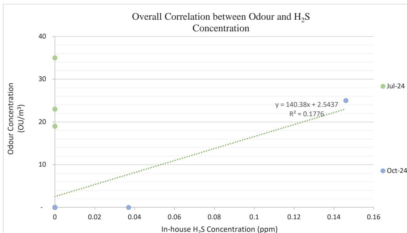
Graph 2 Correlation between Odour and H 2 S Concentration for Jul 2024 and Oct 2024
